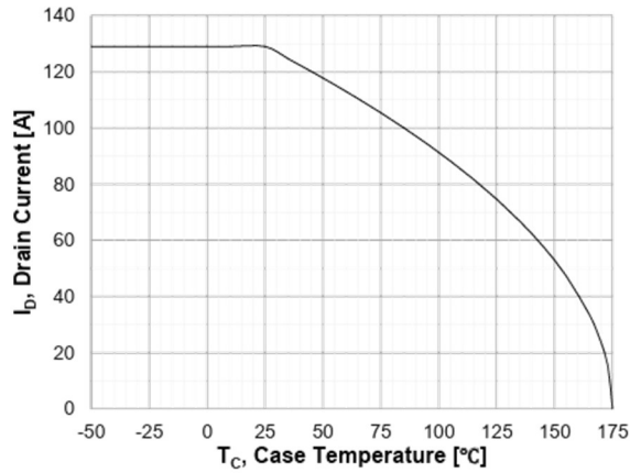
Figure 13. Continuous Drain Current Derating vs. Case Temperature
