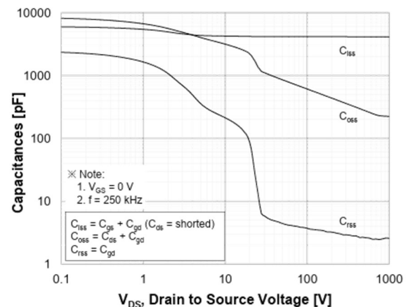
Figure 12. Capacitance Characteristics
