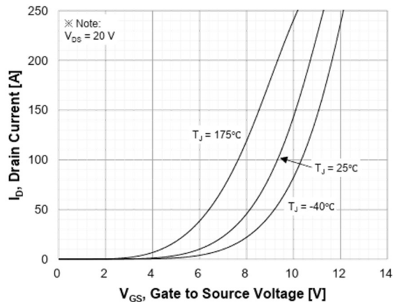
Figure 5. Transfer Characteristic
