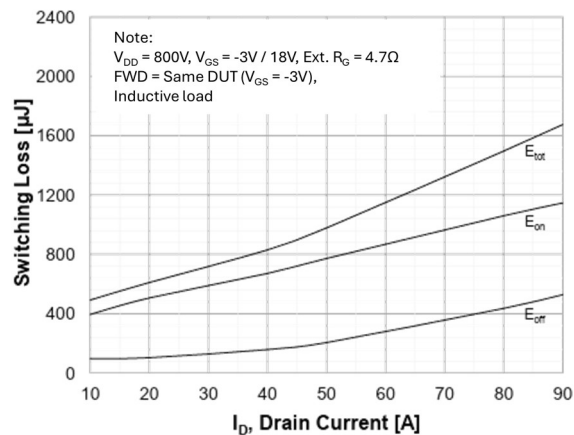
Figure 17. Typical Switching Losses vs. Drain Current
