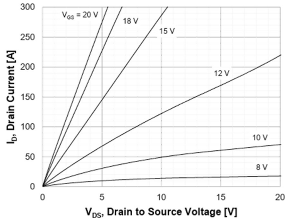
Figure 3. On-Region Characteristics
